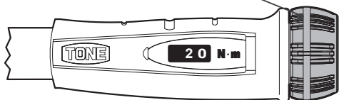
Torque Setting Knob
